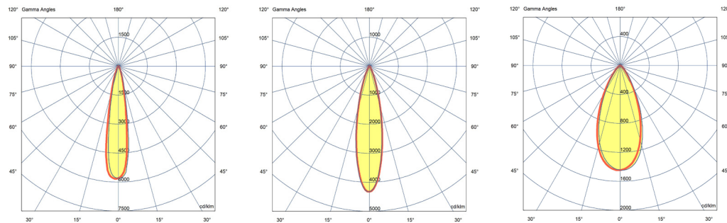
15° beam angle polar curve shown
