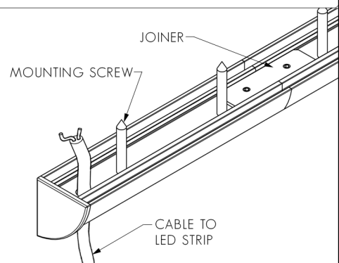
FIG. 2 - TOP VIEW
