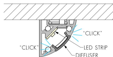
FIG. 3 - ENSURE DIFFUSER IS MOUNTED SECURELY
