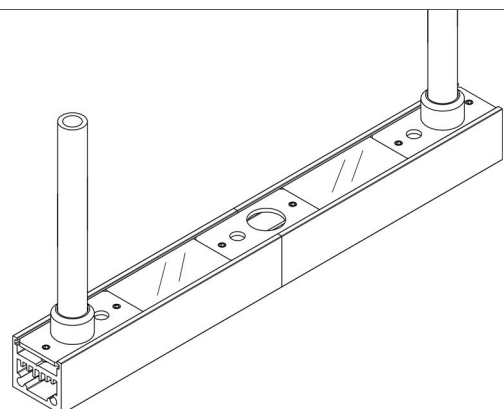
FIG. 3 - ASSEMBLY EXAMPLE
