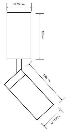
Surface Mounted
