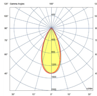
45° beam angle polar curve shown
