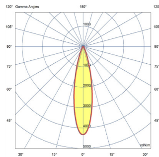
25° beam angle polar curve shown
